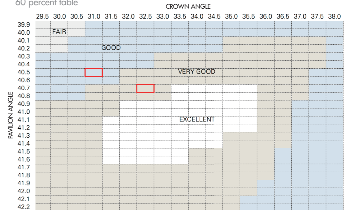
Crown and Pavilion Angle Combination Chart for a Diamond with a 60% Table
